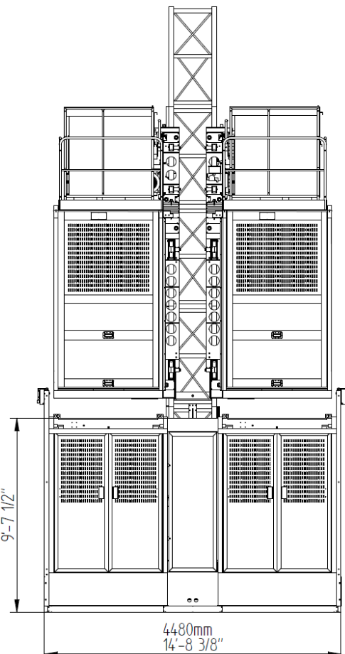
Front view
